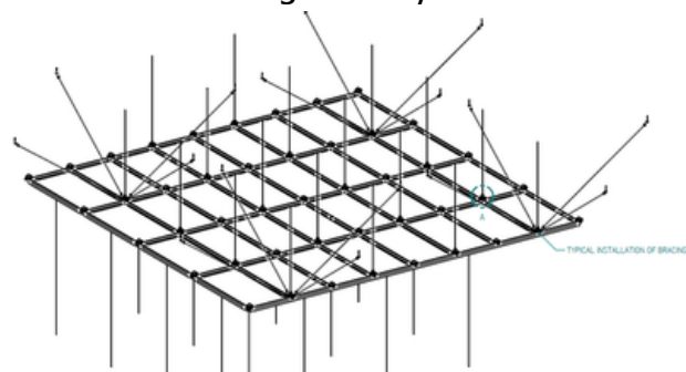
Ceiling Grid System
